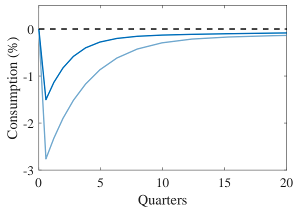
Figure 13: Energy dynamics and aggregate consumption.
